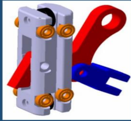
New Design Assembly
